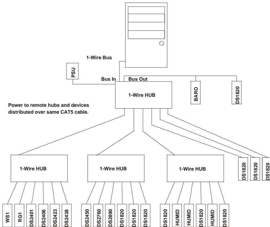
Cascading Branches Topology
